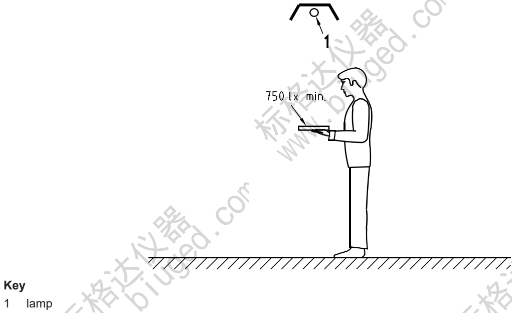
Figure 1 — Configuration of lamp, test panel and observer
