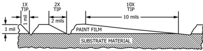
FIG. 2 Grooves Made by 1x, 2x, and 10x Cutting Tips
