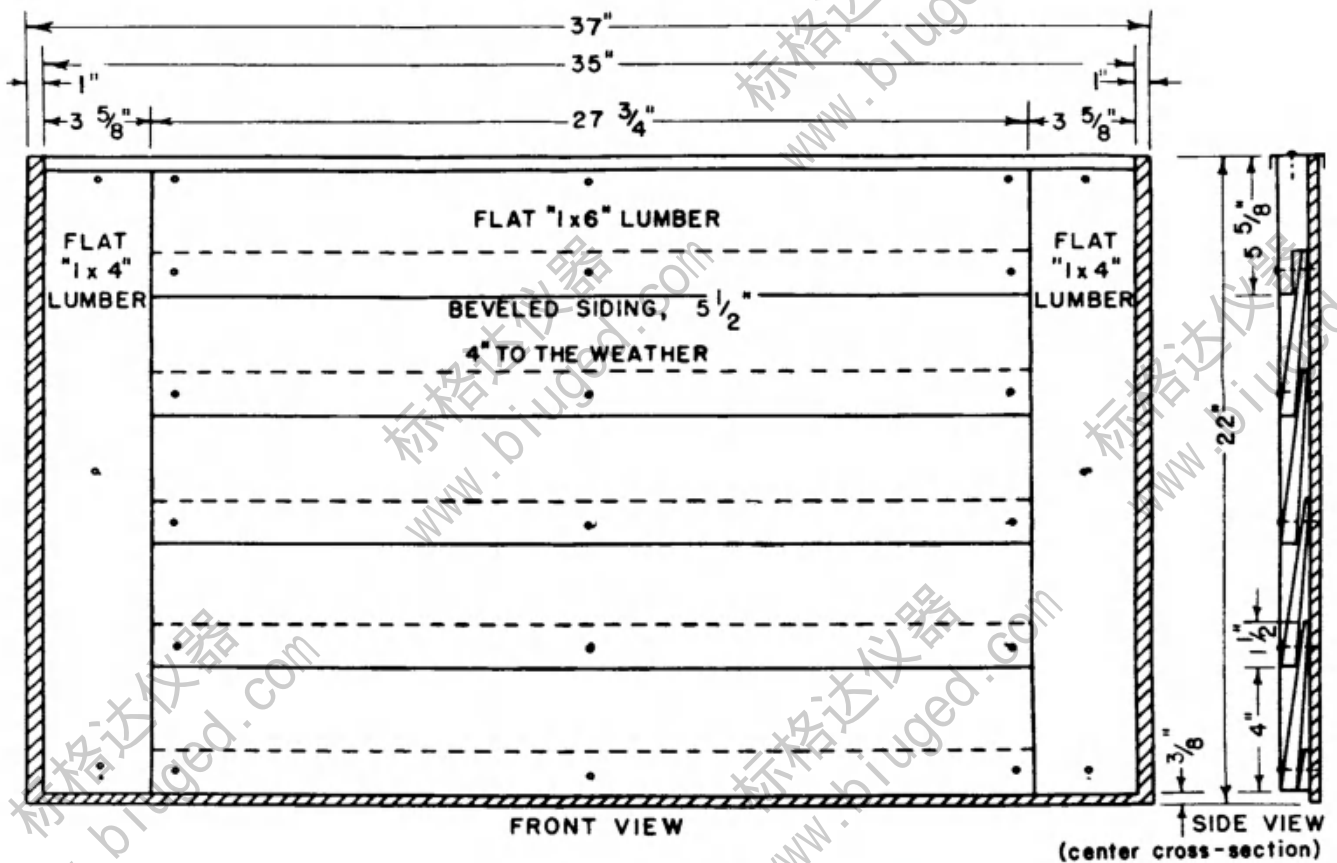
NOTE 1—1 in. = 25.4 mm. FIG. X1.3 ASTM Test Panel for Exterior Exposure of Trim Paints
