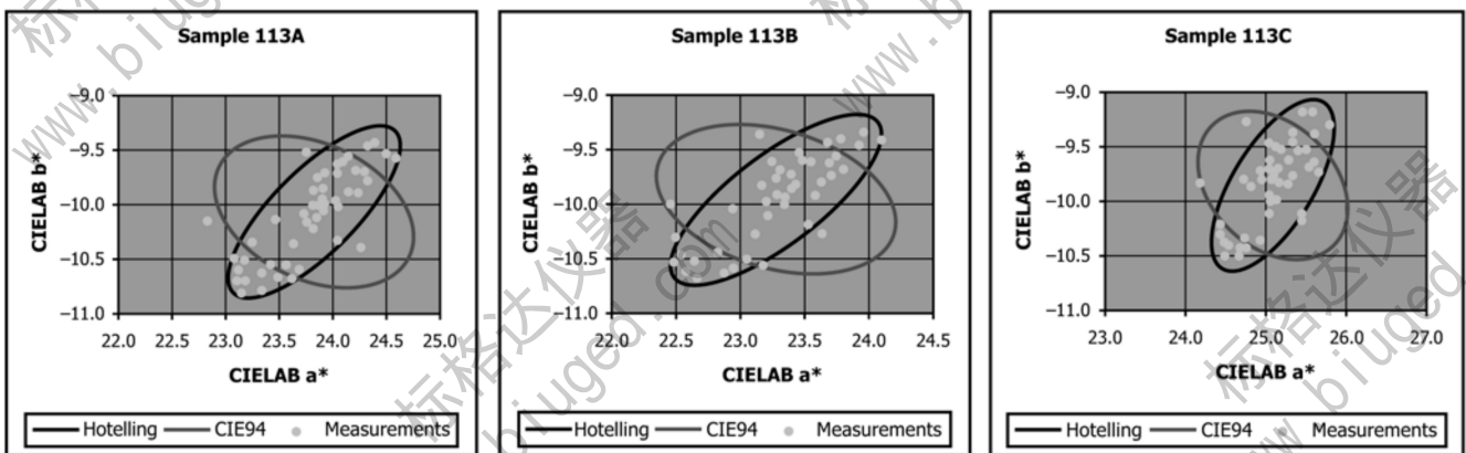
FIG. X1.1 Plots of CIELAV a*-b* for the CRP Reports 113
